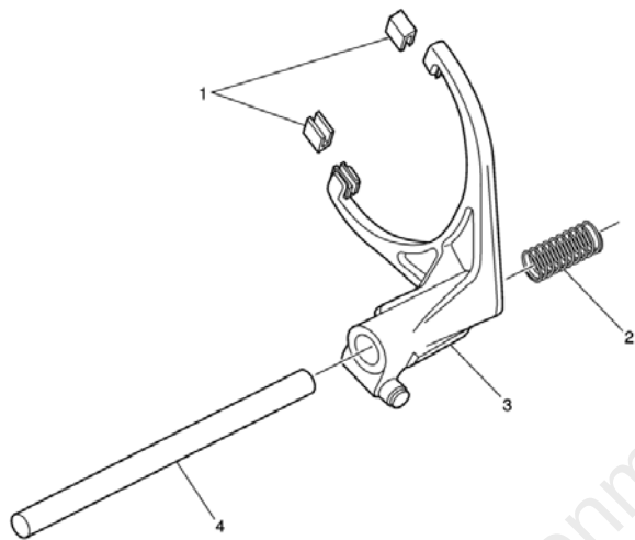
Two/Four Wheel Drive Shift Components Cleaning and Inspection
